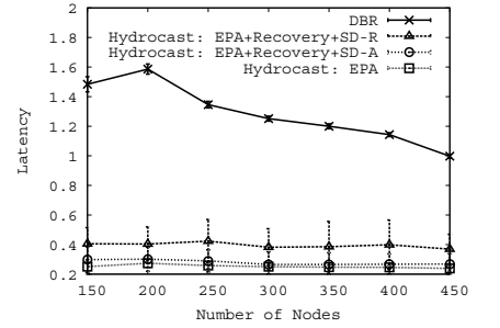
Fig. 13. Average end-to-end delay
