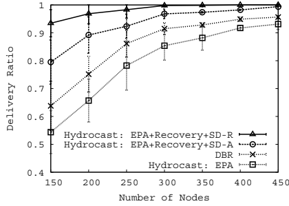
Fig. 11. Packet delivery ratio
